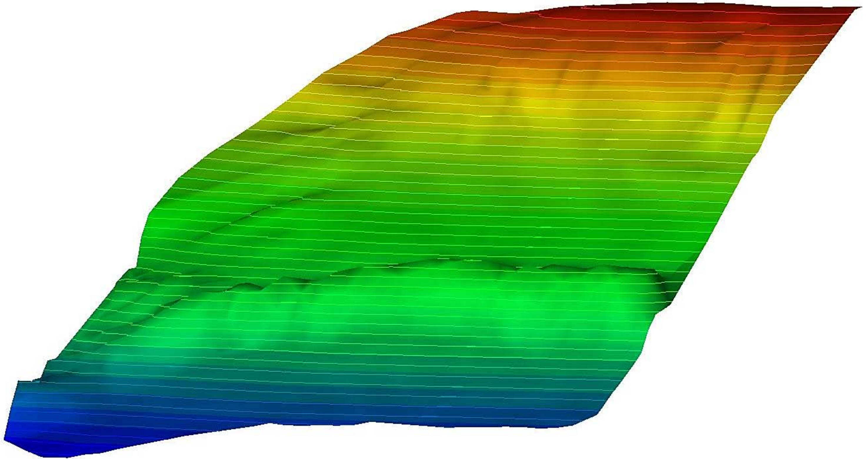
3D INTERPRETATION OF SEA FLOOR SLOPE BAMBOUS 2
